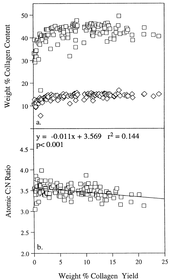
Fig. 1. (a) Collagen carbon ( \square ) and nitrogen ( \diamond ) contents by weight percent plotted against collagen yields by weight percent for all collagenous faunal bone sampled from Rancho La Brea asphalt seeps. (b) Collagen atomic C/N ratios regressed against collagen yields for all collagenous samples.
