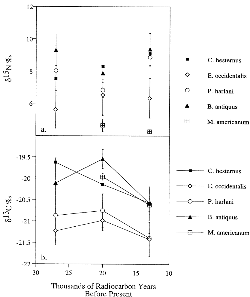
Fig. 5. (a–b) Rancho La Brea species mean \delta^{15}\text{N} and \delta^{13}\text{C} values shown at 1 standard deviation plotted against the age of pits, in radiocarbon years before present, from which samples were recovered. Samples dating to 28–26 ka (terminal OIS 3) are from Pits 60 and 91, samples dating to 20 ka, or last glacial maximum, from Pit 3 and samples dating to 14–12 ka, or the glacial–interglacial transition (GIT), from Pits 61 and 67.
