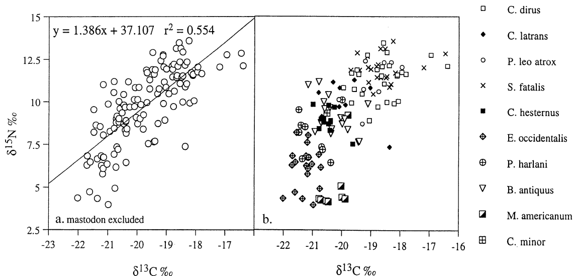
Fig. 3. (a) Rancho La Brea individual \delta^{15}\text{N} values plotted against \delta^{13}\text{C} (mastodon excluded), showing a positive correlation significant at p > 0.0001 . (b) Individual \delta^{15}\text{N} values plotted against \delta^{13}\text{C} by species.
