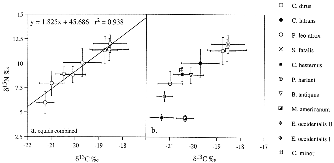
Fig. 4. (a) Rancho La Brea species mean \delta^{15}\text{N} values plotted against mean \delta^{13}\text{C} values at 1 standard deviation (equids combined, mastodon excluded), showing a strong positive correlation significant at p > 0.0001 . (b) Mean \delta^{15}\text{N} values plotted against \delta^{13}\text{C} values by species, shown at 1 standard deviation, mastodon included and equids plotted in two groups.
