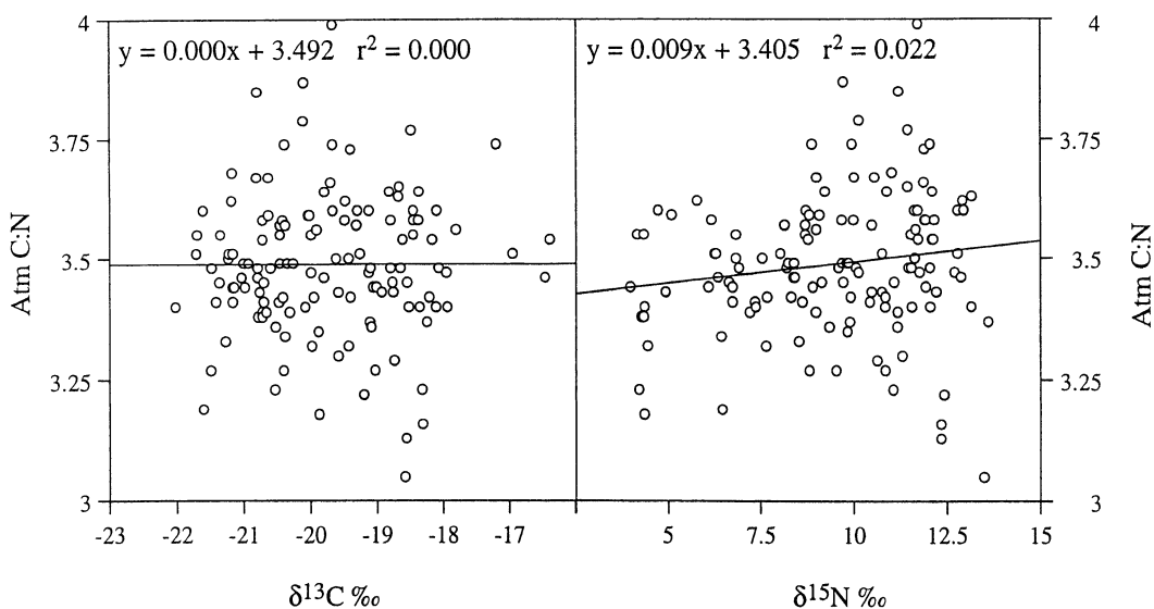
Fig. 2. Rancho La Brea atomic C/N ratios plotted against \delta^{13}\text{C} and \delta^{15}\text{N} values with correlation coefficients.
