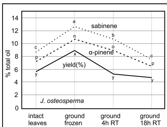
Fig. 7. Changes in oil yield, \alpha -pinene, and sabinene (% total oil basis).
