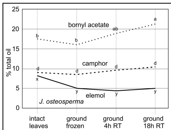
Fig. 9. Variation in bornyl acetate, camphor and elemol (% total oil basis) among treatments.
