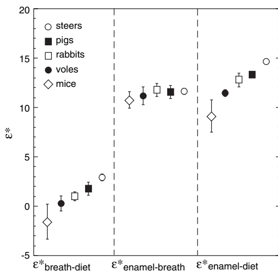
Fig. 1. Single axis plot of epsilon values for different species. Mice data are from Tieszen and Fagre [36].
