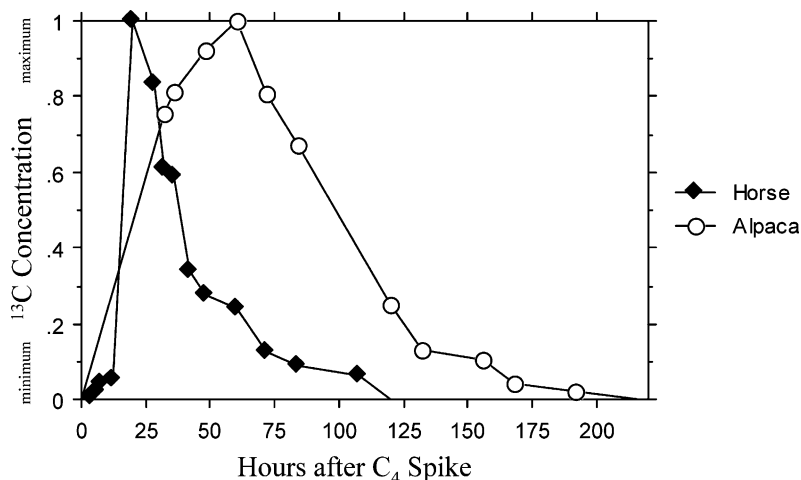
Fig. 1. Stable carbon isotope excretion curves for one horse and one alpaca. Transformed stable isotope concentration data are represented on y-axis and hours after the C 4 spike on the x-axis.
